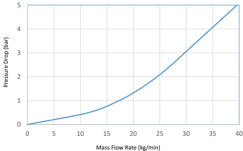
0 - 40 kg/min water, sensor with P1 pressure rating. Higher viscosities create higher pressure drop
